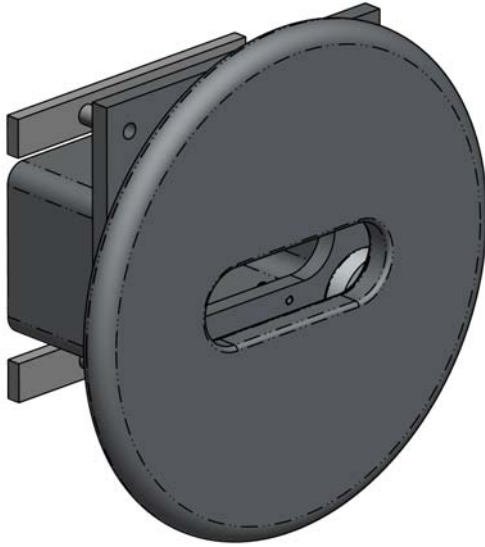
High Current Post Accel Extraction Assembly
