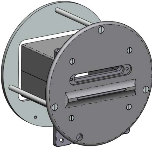
High Energy Extraction Head, Selective Aperture Assembly
