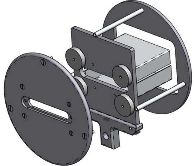
Glemco Modified HE Manipulator Head
