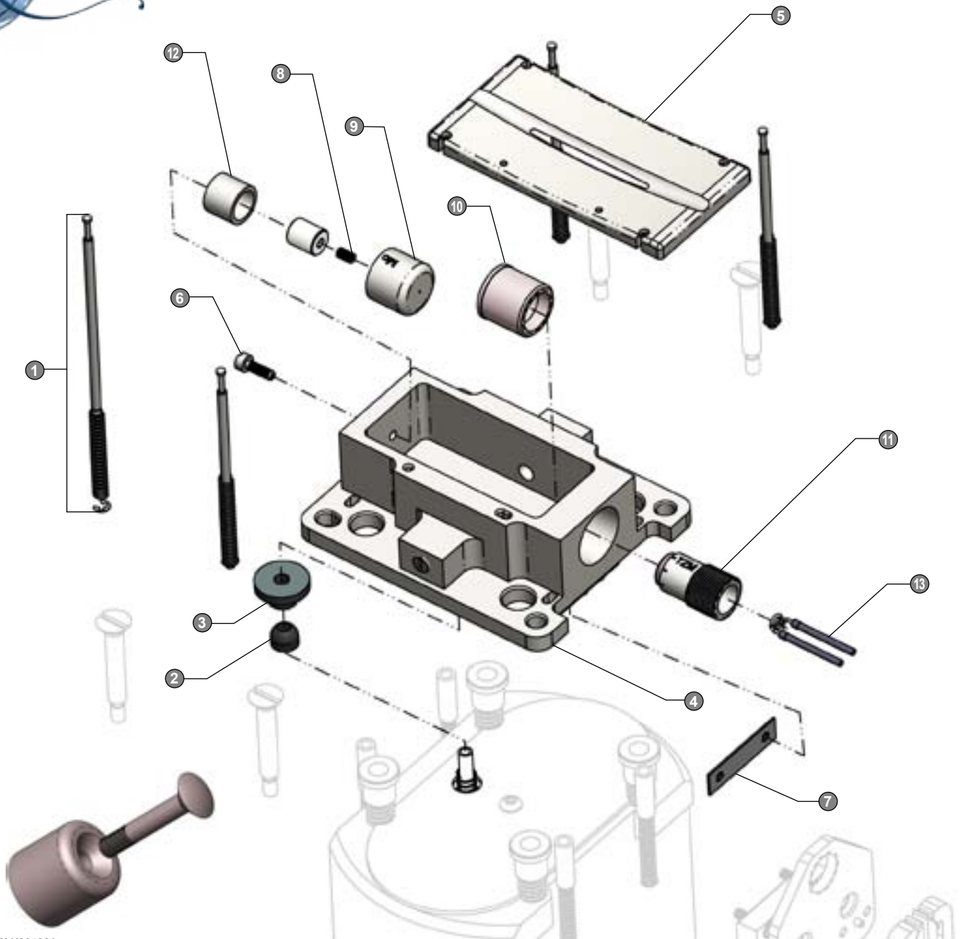
P/N K99430A Glemco also offers a 2 PC Cathode Assembly Kit. Contact sales for more information.
