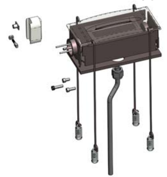
Varian VISta™ HCP Assembly pg. 4
