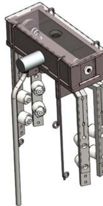
Varian VISta™ 810 Bernas Source Assembly pg. 7
