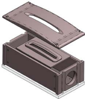
Varian VISta™ HCP Assembly pg. 5
