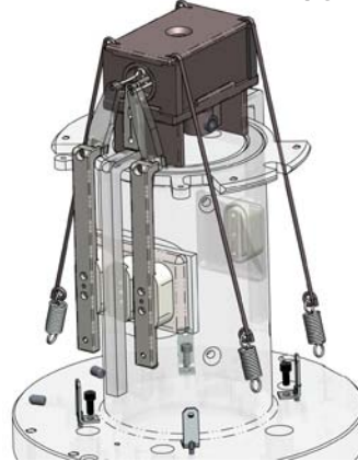
Varian VISta™ 810 Ion Source pg. 3
