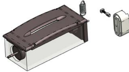
Varian VISta™ HC / IHC Source pg. 2
