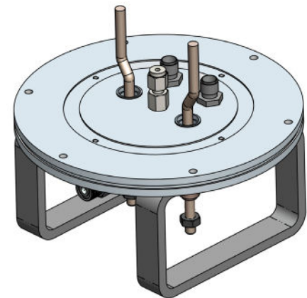
P/N 20902 MC200 Source Plate Assembly
