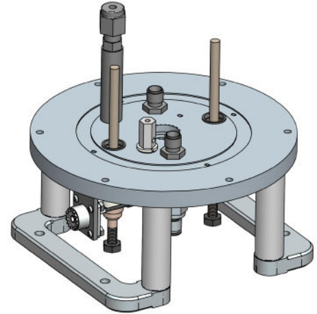
P/N 10611A Source Plate Assembly
