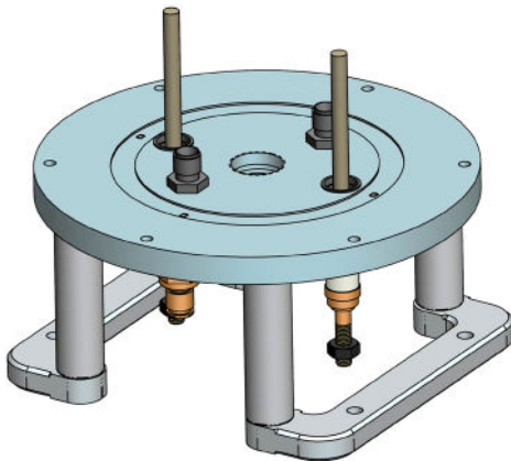
P/N 10611 OEM 0342-0563-3001 Source Plate Assembly
