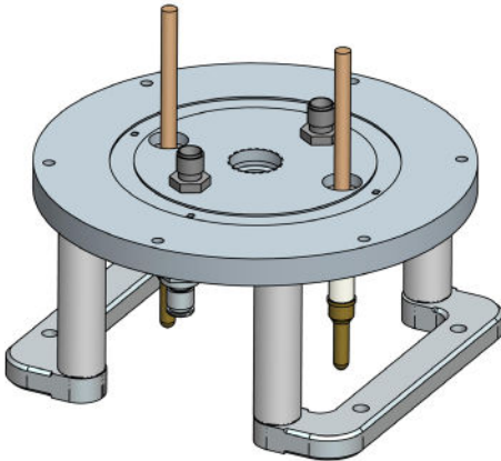
P/N 10625 6200AV Source Plate Assembly Utilizes "Slip-On" Power Feedthru Adapters, Used With Glemco Cable Assembly (P/N 10631)
